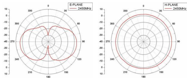
E-Plane Field Pattern
